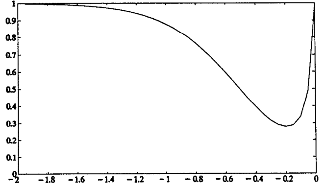
FIG. 5. Plot of H(x) of the third example.
