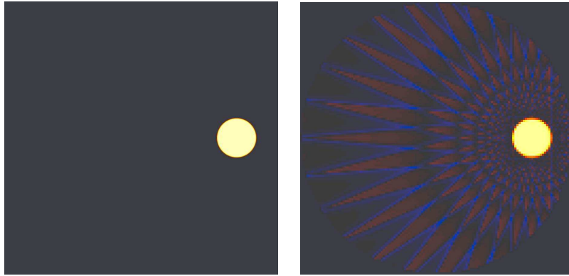
Figure 7: Few projections (20 proj)
