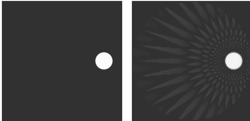
Figure 8: Few projections (20 proj)
