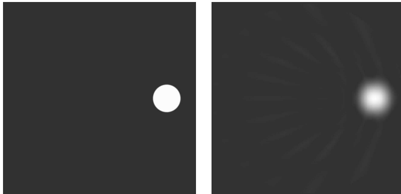
Figure 6: Insufficient sampling in p
