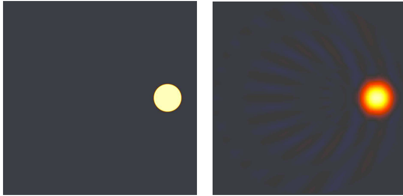
Figure 5: Insufficient sampling in p
